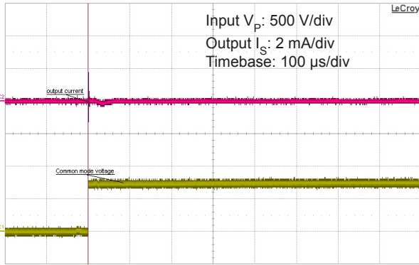
Figure 11: Typical common mode perturbation (750 V step with 6 kV/μs R_M = 100 \Omega )
